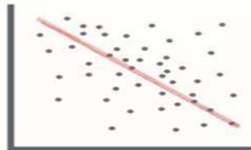
Negative Correlation
