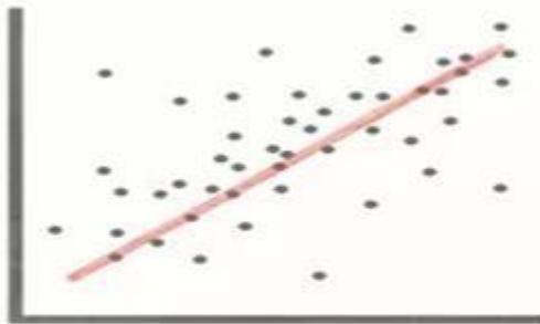
Positive Correlation
